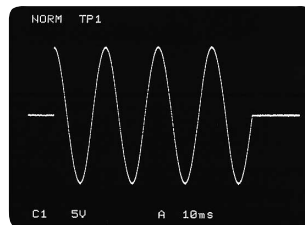
Output ON/OFF Phase Setting Output on phase: 90 deg. Output off phase: 0 deg
